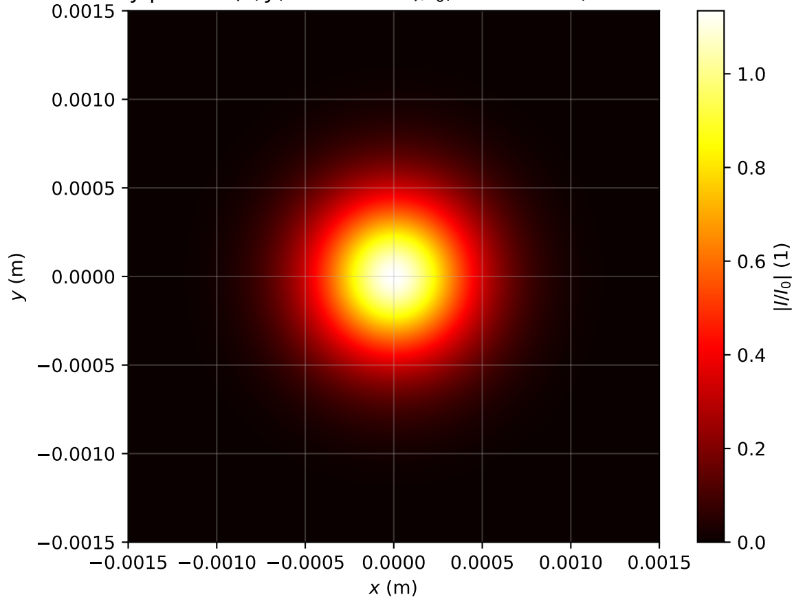
Intensity profile I(x, y, z = 0.478m)/I_0 , P_{in}=0.9P_{cr} , artificial time
